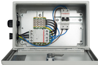
CONTROL BOX (3 * 400 V / 3*480V)
