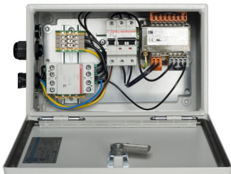
CONTROL BOX (3 * 400 V / 3*480V)
